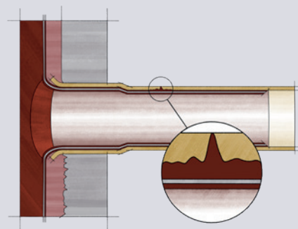
plastocor® Inlet System for tube end inlet & outlet protection
