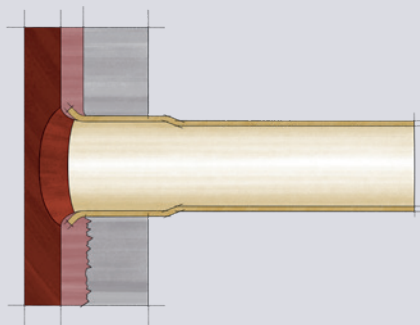
plastocor® Cladding System for tube sheet protection
