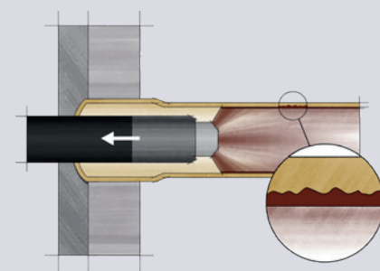
plastocor® Tube Lining System for full-length tube protection
